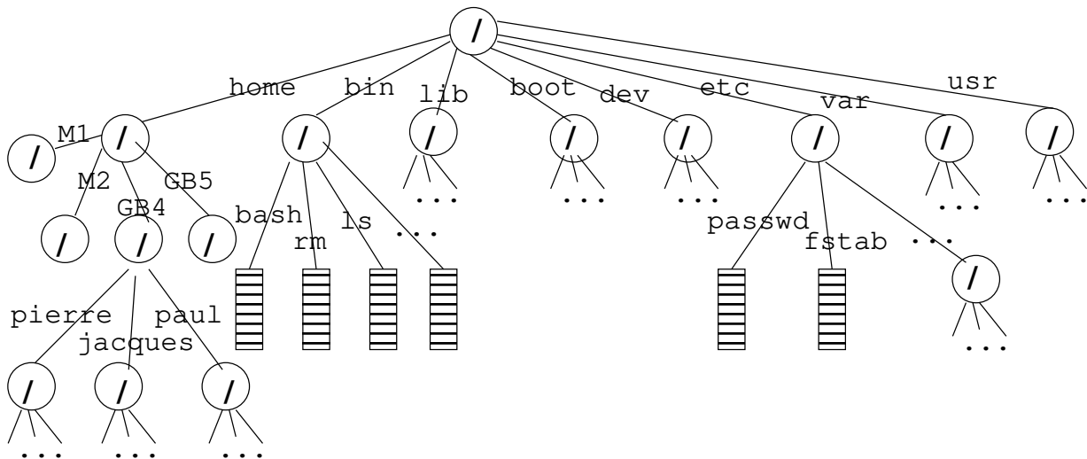
FIGURE 1 – Arborescence UNIX
