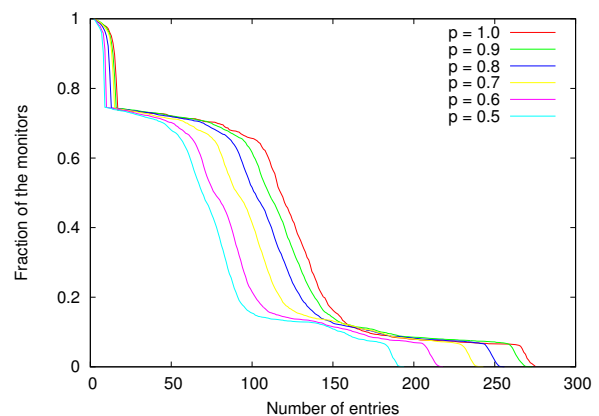
Fig. 6. Inverse cumulative distribution of the number of entries in the AS prefixes table for several monitors subset sizes.
