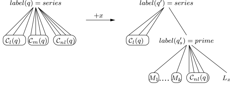
Figure 3: Updating the modular decomposition tree when the insertion node is a series node. The modules M_1 \dots M_k are the maximal uniform modules of G[Q_s]
