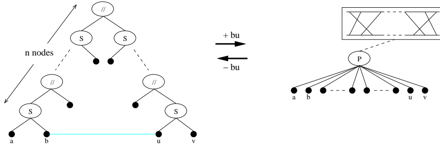
Figure 2: An edge insertion/deletion implying O(n) changes in the full modular representation. When the edge bu is inserted in the cograph whose decomposition tree is given on the left, it becomes prime and remains a permutation graph. The number of nodes in its modular decomposition tree switches from 2n - 1 to 1. Conversely, when the edge bu is deleted in the prime permutation graph represented on the right, it becomes a cograph.
