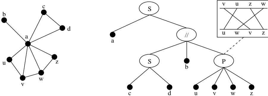
Figure 1: A permutation graph and its full modular representation.
