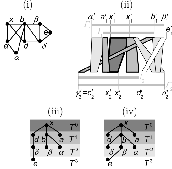
Figure 3: A trapezoid graph (i), its trapezoid model (ii) labeled as in the beginning of the second iteration of the main loop of Algorithm 1, and two BFS trees: one respecting priority order (x\beta\delta dbea\alpha) (iii) and the other respecting priority order (x\beta\delta bdeaa) (iv).
