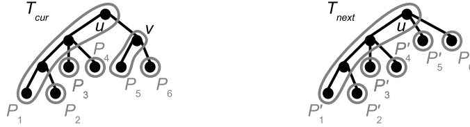
Figure 3: Left: a tree T_{\text{cur}} with its path partition \mathcal{P}_{\text{cur}} = \{P_1, P_2, P_3, P_4, P_5, P_6\} whose partition tree T_p^{\text{cur}} has height 2. Right: the tree T_{\text{next}} resulting from the contraction of edge uv in T_{\text{cur}} , together with its path partition \mathcal{P}_{\text{next}} = \{P'_1, P'_2, P'_3, P'_4, P'_5, P'_6\} . All the paths in \mathcal{P}_{\text{next}} are the same as those in \mathcal{P}_{\text{cur}} , except P'_5 which has lost node v . The height of T_p^{\text{next}} decreased, it is now 1.
