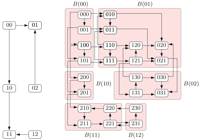
Fig. 8 Asynchronous transition systems ATS(G_1, p_{12}) (left) and ATS(G_2, p_2) (right)
