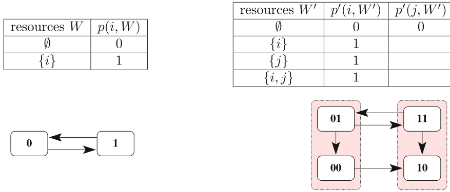
Fig. 11 a G' -model p' (right) and its reduced G -model p (left)
