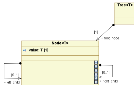
Figure 5: Structure de l'arbre binaire, version templated
