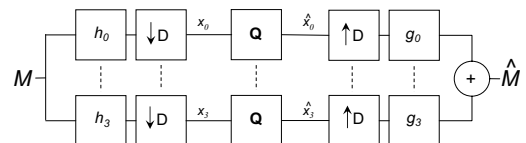
Figure 2: Principle of a 4-channel wavelet coder.
