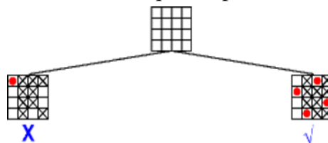
Fig. 9.1b: Search tree for the four queens problems with weak propagation
