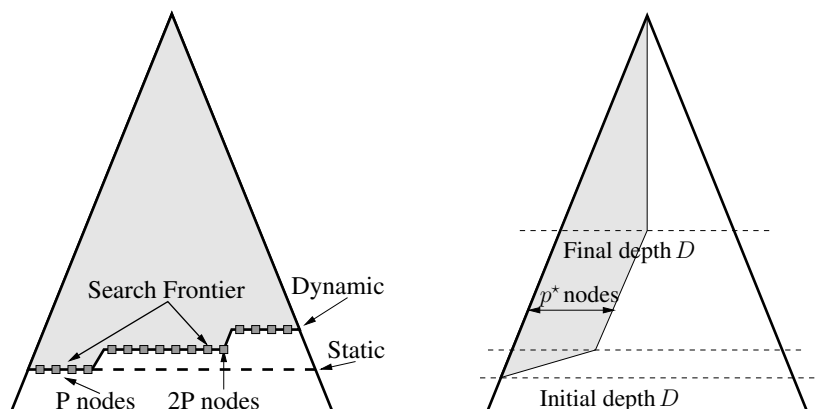
Fig. 9.7: Bottom-up decomposition and estimation
