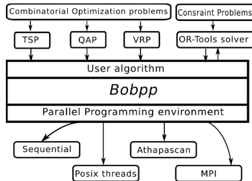
Fig. 9.2: Bobpp framework
