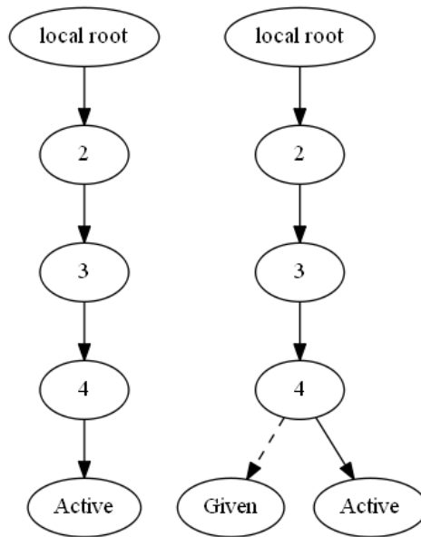
Fig. 9.3: Simple work separation
